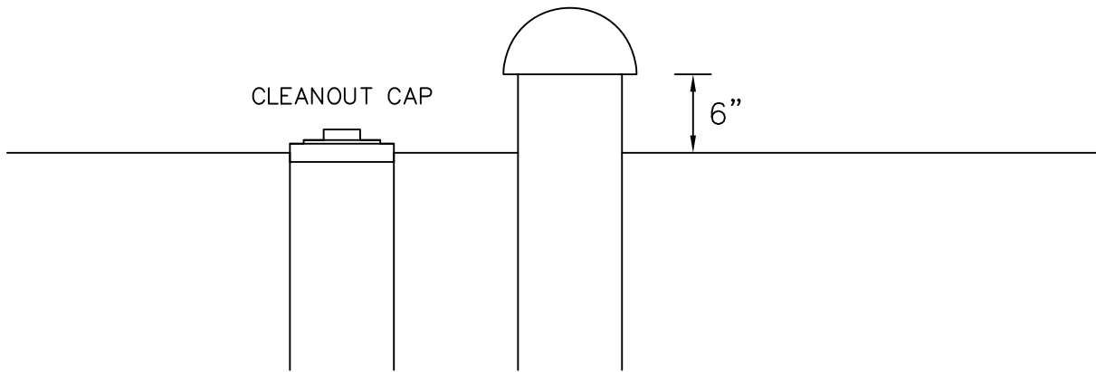
VENT W/ MUSHROOM CAP
